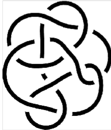
Conway knot
