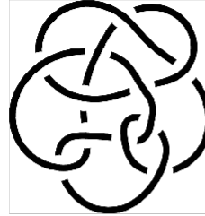
Kinoshita-Terasaka knot
